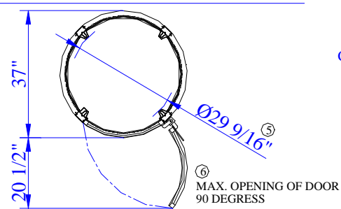
VIEW "A-A"
